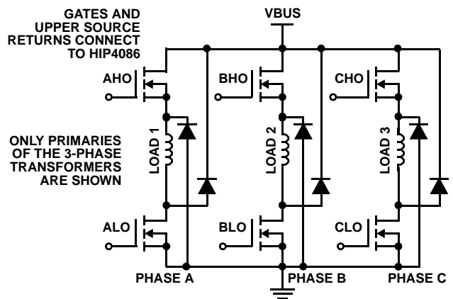
FIGURE 7. DOUBLE-FORWARD CONVERTER BRIDGE CONFIGURATION
