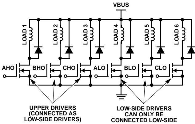
FIGURE 6. 6-LOWER CONFIGURATION
